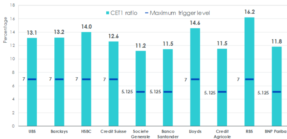
Figure 4 - Top 10 AT1 CoCo issuers - capital ratios
