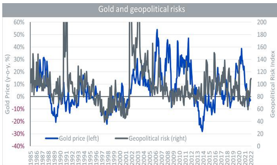
Figure 2: Gold and geopolitical risks
