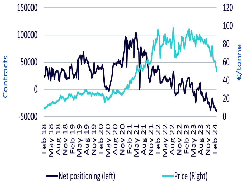
Figure 2: Investment fund net positioning and price of EUAs
