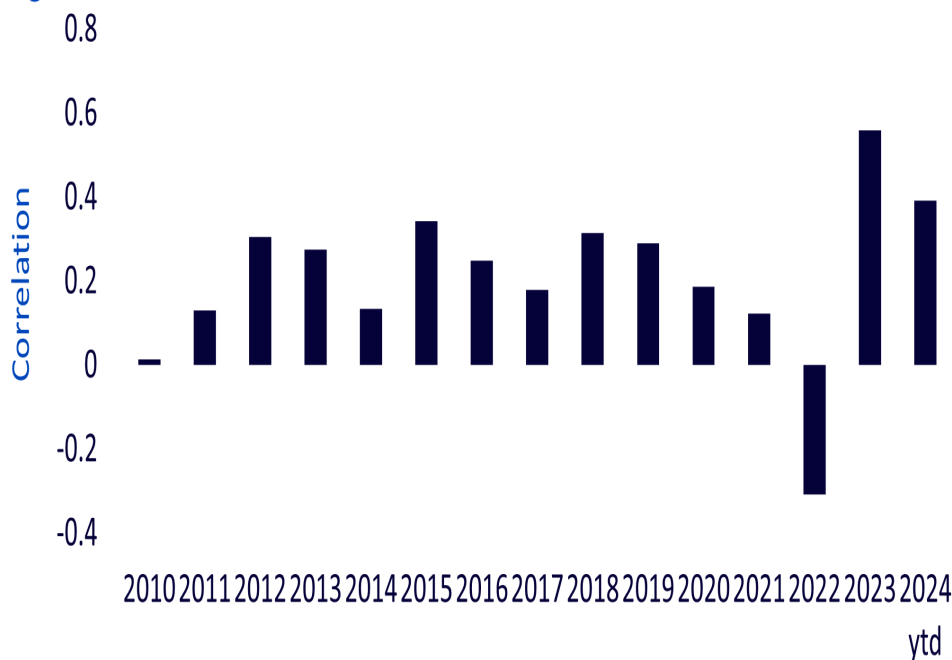
Figure 1: Correlation between EUAs and TTF
